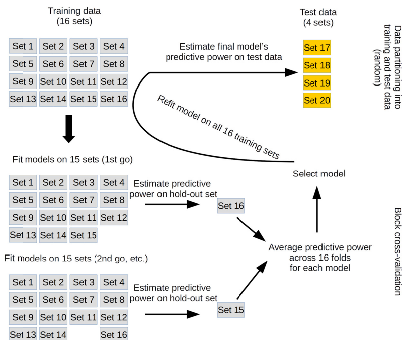
Figure 3. Illustration of how the data were partitioned into a training and a test set and of how block cross-validation works. Only two iterations of block cross-validation are shown; in reality, sixteen took place for each model. Each ‘Set’ refers to 50-52 texts that were rated by a panel of judges. The panels of judges for different sets did not overlap.
